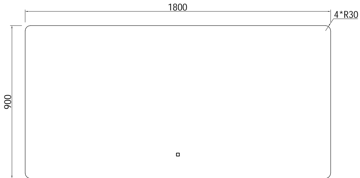
Front View
