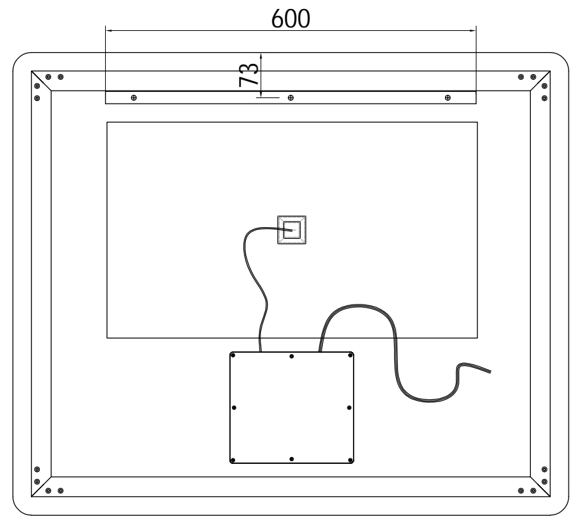
rear view
