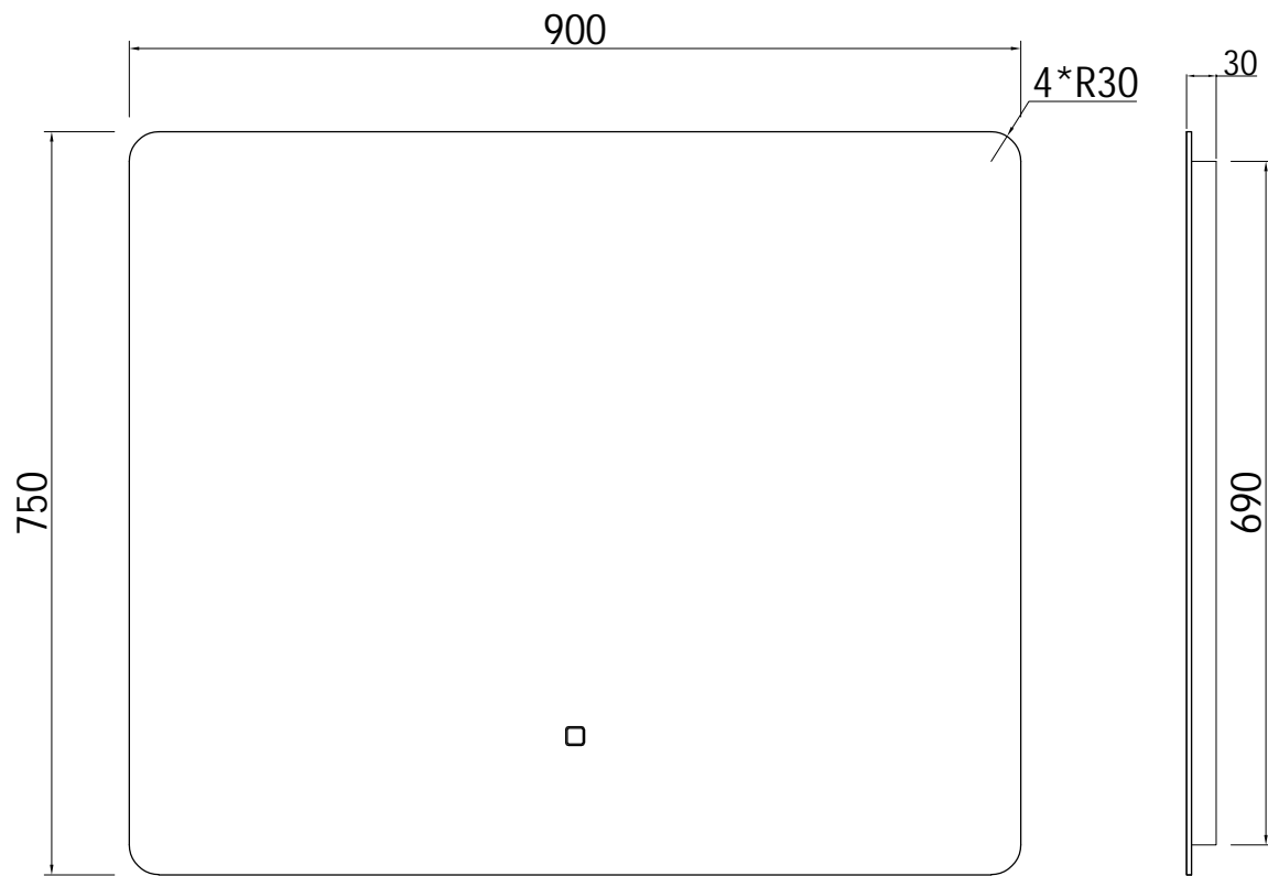
front view
