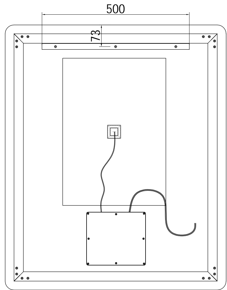
rear view
